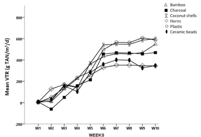
Fig. 4. Mean volumetric TAN conversion rate ( \text{g TAN}/\text{m}^3/\text{d} ) demonstrated by different biomedia in different experimental period.
