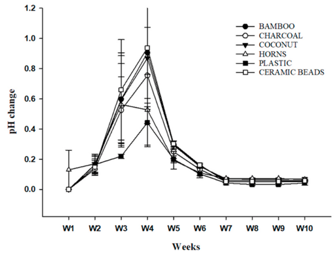
Fig. 1. Change in pH during single passage over different biofilters. The changes were measured as influent pH – effluent pH.
