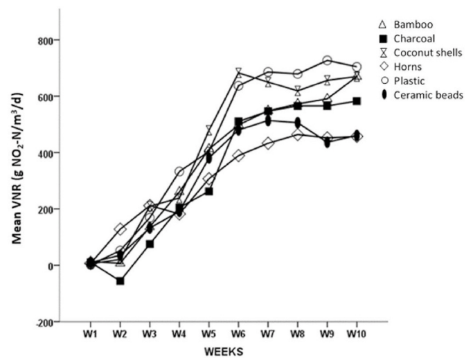
Fig. 6. Mean volumetric nitrite conversion rate (g NO 2 -N/m 3 /d) demonstrated by different biomedica in different weeks of the experiment.
