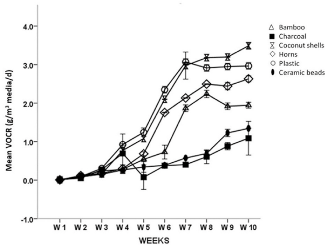
Fig. 3. Mean volumetric oxygen conversion rate in \text{g}/\text{m}^3/\text{d} observed in different biomedia at time of the experiment (calculated as dissolved oxygen in – dissolved oxygen out).
