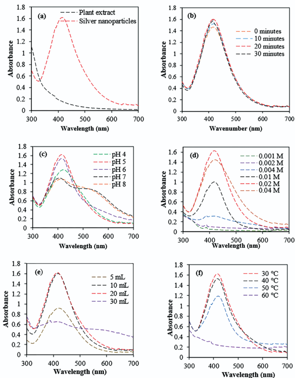
Figure 2: UV-Visible absorption spectra of ssynthesised ZPLAgNPs showing resonance peak at 420 nm (a) as a function of reaction time (b), pH of reaction (c), \text{AgNO}_3 concentration (d), extract volume (e), and reaction temperature (f).
