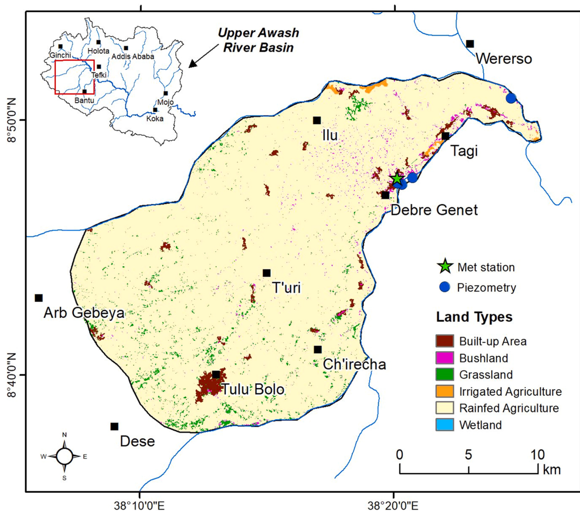
Fig. 4. Map of land cover of the Upper Awash observatory of south-central Ethiopia (Chandrasekharan et al., 2021); the position of this sub-catchment area (446 km 2 ) is indicated in the inset drainage map, headwaters of the River Awash Basin.
