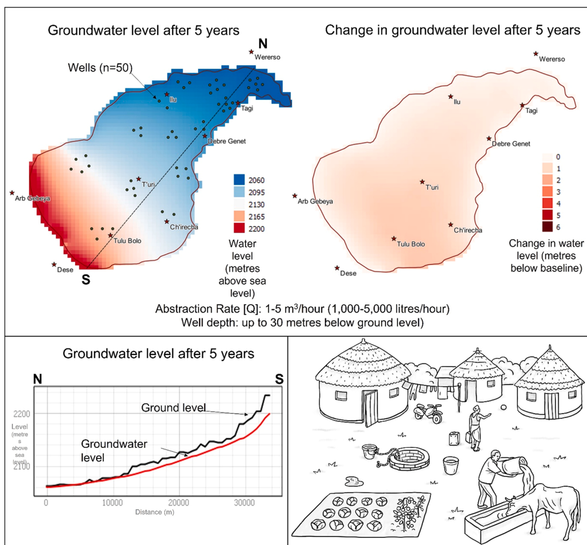
Fig. 6. Examples of choropleths and cross section showing change in groundwater levels after five years, and image, shown on posters and pamphlets for Ethiopia representing the 'small-scale multi-use' pathway.
